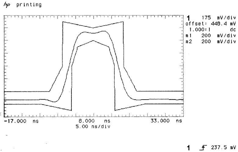
Figure 3-9 34 Mb/s Isolated Positive Pulse
