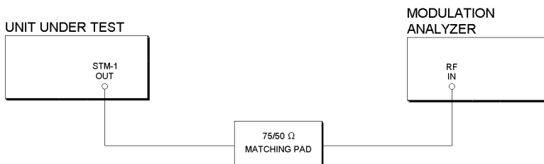
TX Jitter Accuracy Test Setup SDH Range 50
