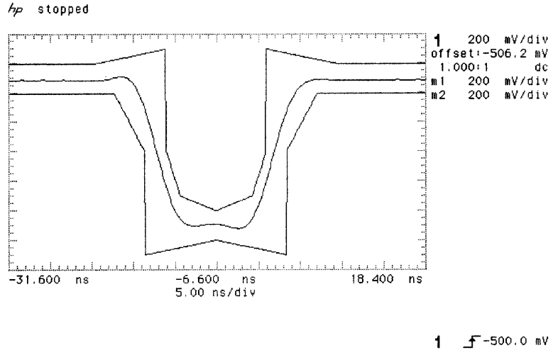
Figure 3-10 34 Mb/s Isolated Negative Pulse
